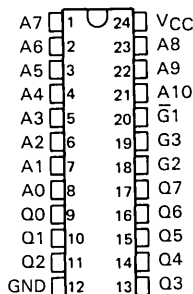
TBP38SA165 . . . JT OR NT PACKAGE TBP38SA166 . . . JW OR NW PACKAGE (TOP VIEW)
