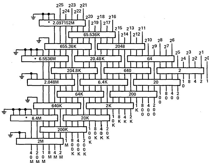
27-BIT-BINARY-TO-BCD CONVERTER
