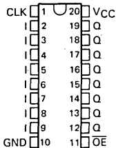
THCTPAL16R8-M . . . J PACKAGE THCTPAL16R8-C . . . J OR N PACKAGE (TOP VIEW)
