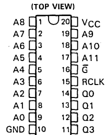
TBP34R162 . . . J OR N PACKAGE
