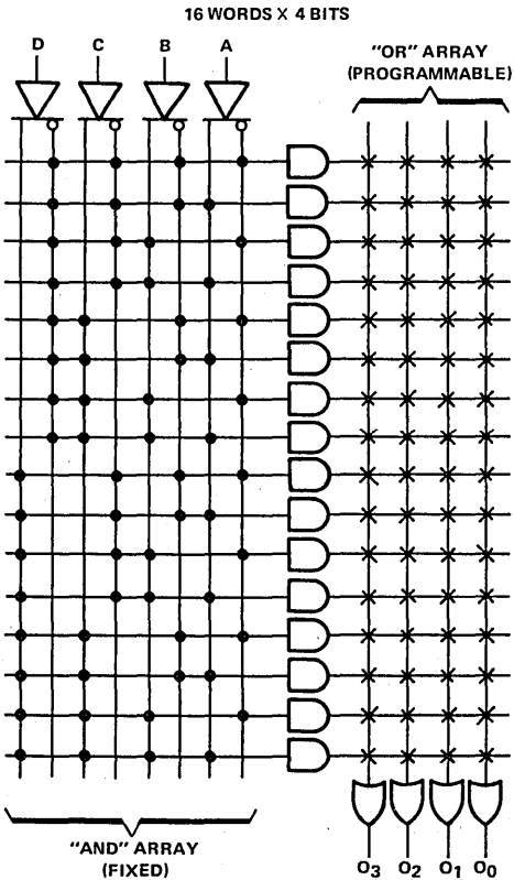
Figure 3. PROM Architecture
