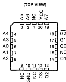
TBP34S1X, TBP34L1X, TBP34SA1X FN OR FK PACKAGE
