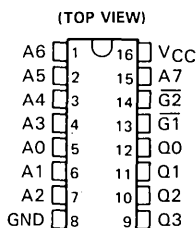
TBP34S10, TBP34L10, TBP34SA10 N OR J PACKAGE
