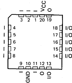
TIBPAL16L8' C SUFFIX . . . FN PACKAGE (TOP VIEW)
