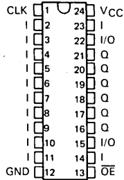
TIBPAL20R6' M SUFFIX . . . JT PACKAGE C SUFFIX . . . JT OR NT PACKAGE
