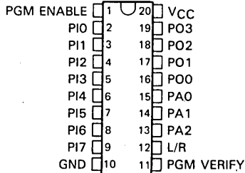
PRODUCT TERMS 0 THRU 31 (TOP VIEW)
