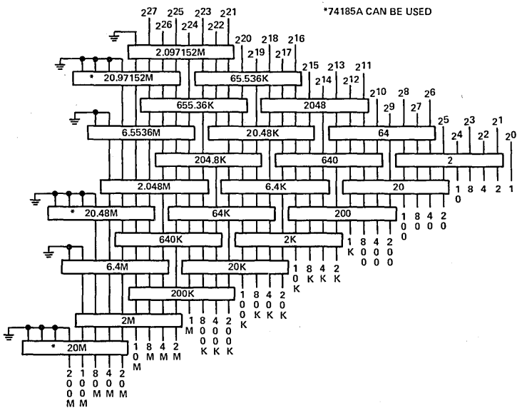
28-BIT-BINARY-TO-BCD CONVERTER
