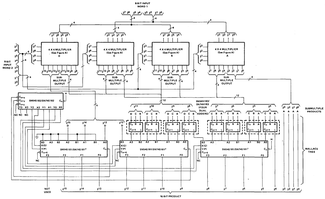
FIGURE B-8 X 8 MULTIPLIER
