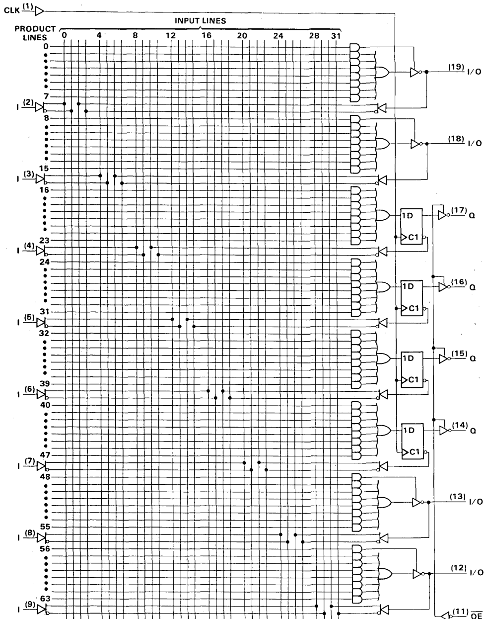
logic diagram
