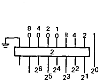
2-DECADE- BCD-TO-BINARY CONVERTER
