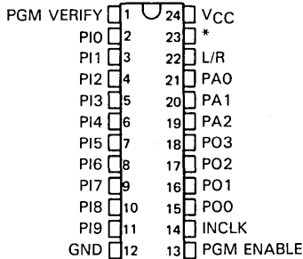
JW OR NT PACKAGE (TOP VIEW)
