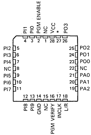
FN PACKAGE (TOP VIEW)
