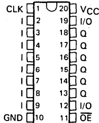
TIBPAL16R6' C SUFFIX . . . J OR N PACKAGE (TOP VIEW)
